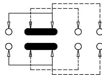
SCHMATIC (SHORTING)
