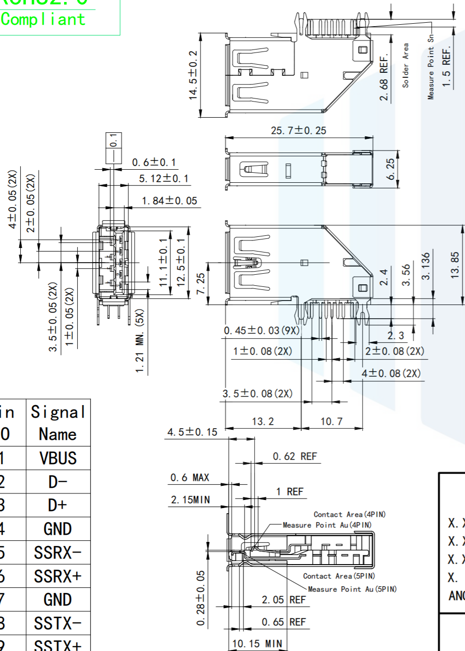
RECOMMENDER P.C.B. LAYOUT TOP VIEW (COMPONENT SIDE TOLERANCE ± 0.05)
