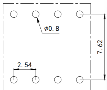
RECOMMENDED P. C. B LAYOUT ( \pm 0.05 )
