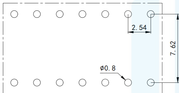
RECOMMENDED P. C. B LAYOUT ( \pm 0.05 )
