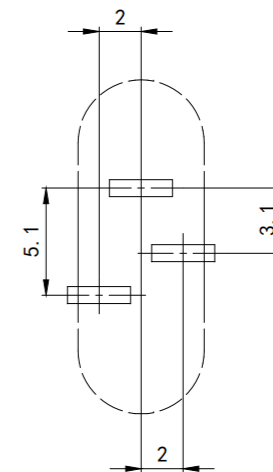
The size of the circuit board cutout
